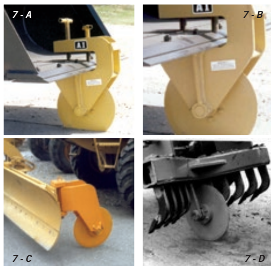
7. A-2b ASPHALT CUTTERS: The strongest cutters available - no other manufacturer even comes close. Our competitors use automotive hubs. These hubs and bolts literally wear off. Attachments International's axle and hub is the strongest ever designed.
