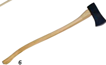
6. H-7 SINGLE BIT MICHIGAN PATTERN AXE: 3 1/2" lb., 8" forged head. 3" ground cutting edge. 36" lacquered hickory handle. • H-7 Single Bit Michigan Pattern Axe
